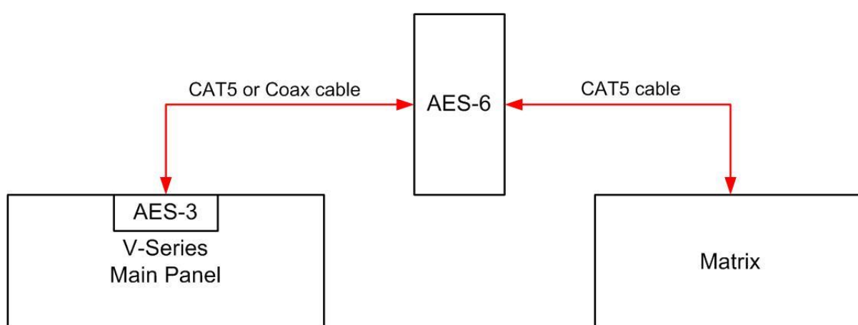
Figure 4-18: V-Series panel with AES-3 connection
