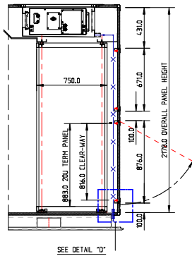
DETAIL OF TYPICAL AUDIO WALL BUILD-UP
